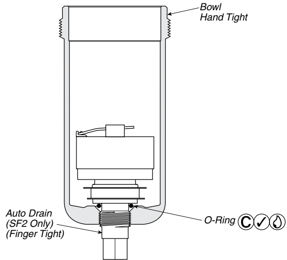
SF2 Metal Bowl w/ Auto Drain
