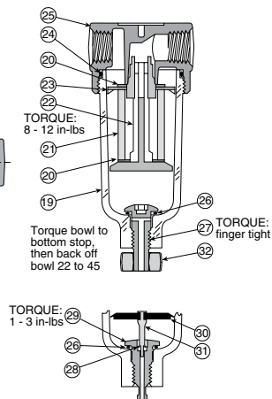
Figure 2: Particulate Filter
