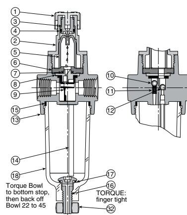
Figure 1: Mist Lubricator
