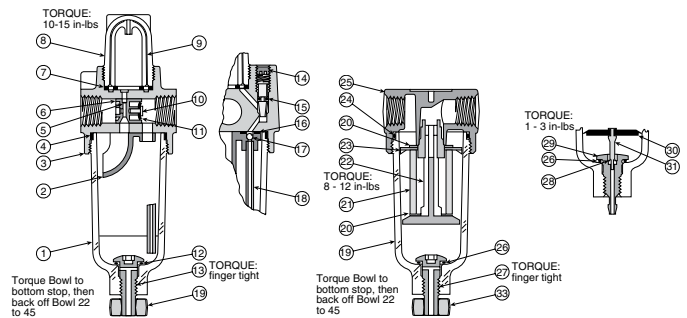
Figure 1: Micro-Mist Lubricator
